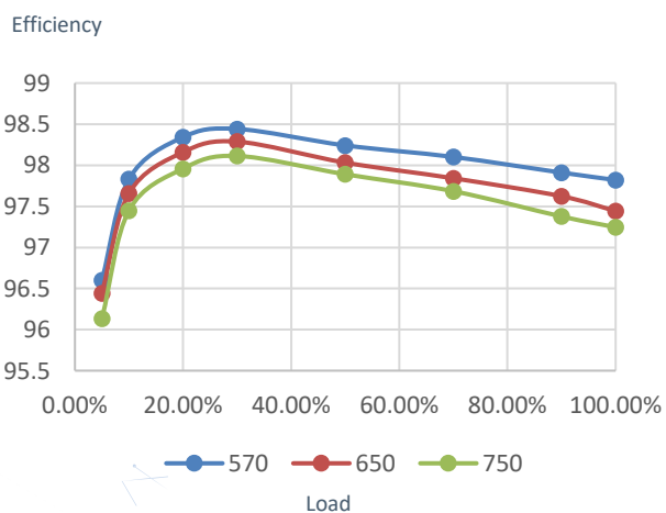
Efficiency Curve
